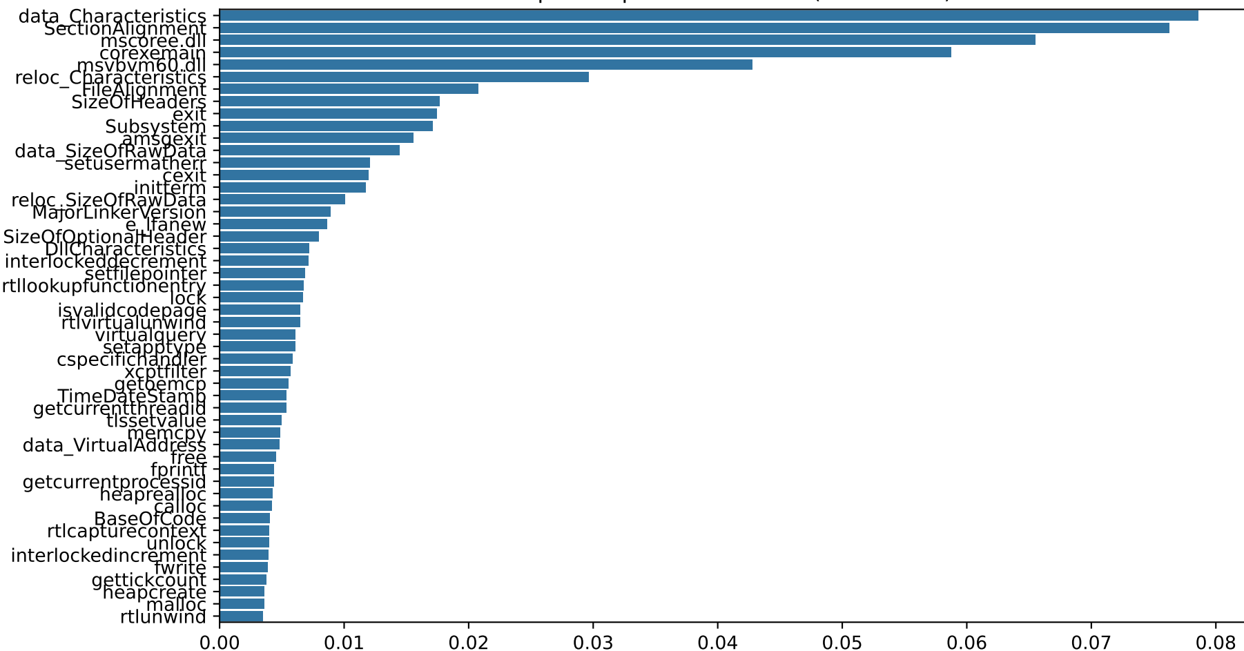
Top 50 Important Features (Extra Trees)
